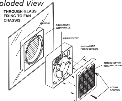
Exploded View
